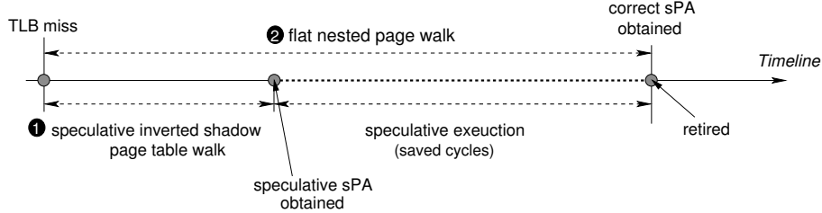
Figure 7: Speculative page table walk with SpecISP
